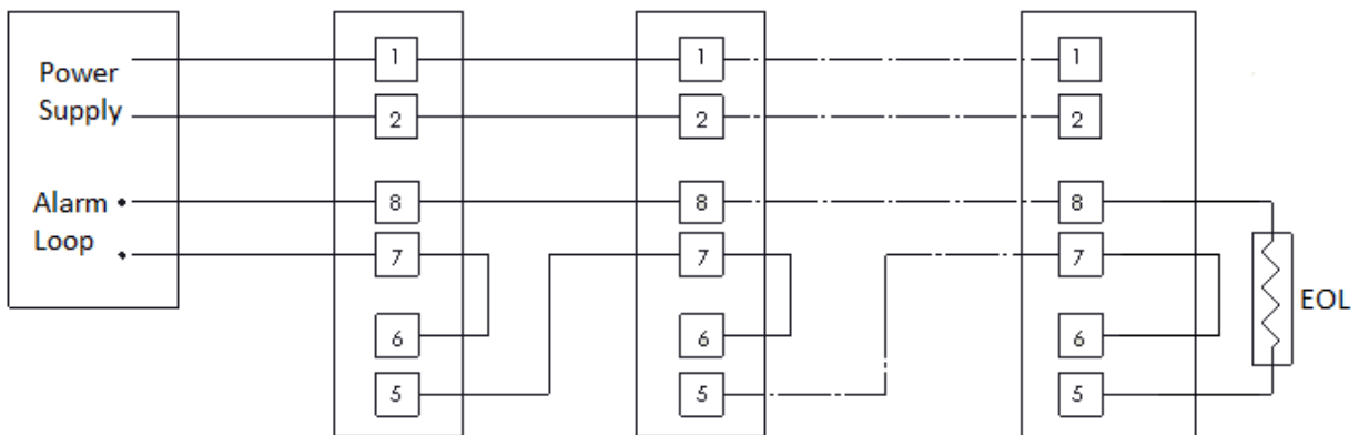
FIGURE 21 – 4 WIRE RELAY CONNECTION
