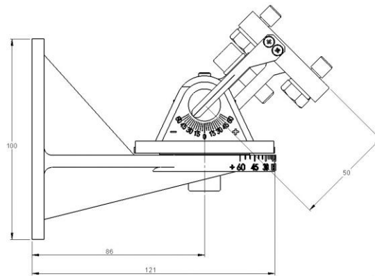
Figure 13 – Tilt Mount Base - Plate View
