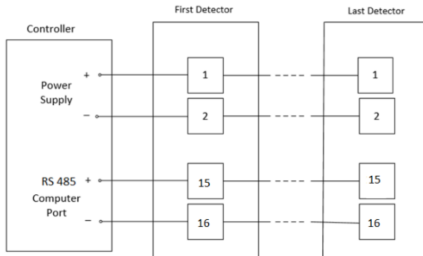
Figure 22 – RS-485 Networking
