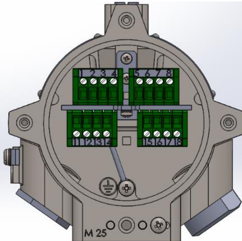
FIGURE 16 – TERMINAL VIEW
