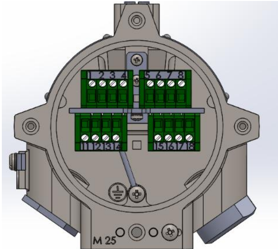
FIGURE 16 – TERMINAL VIEW
