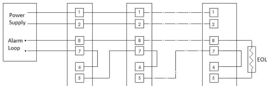
FIGURE 21 - 4 WIRE RELAY CONNECTION
