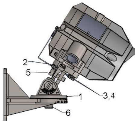
FIGURE 15 - DETECTOR ON TILT MOUNT – SIDE VIEW
