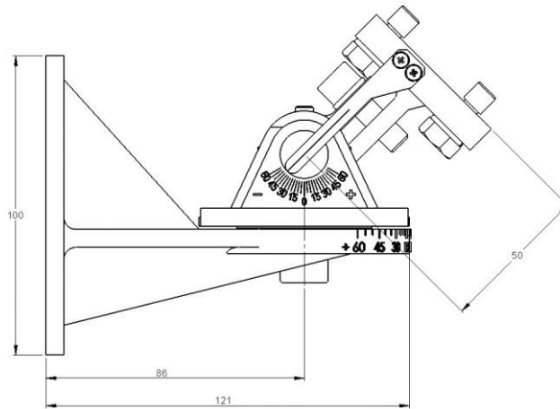
Figure 13: Tilt Mount Base - Front View
