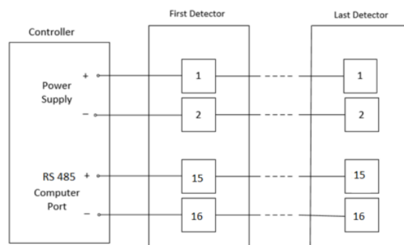
Figure 22: RS-485 Networking
