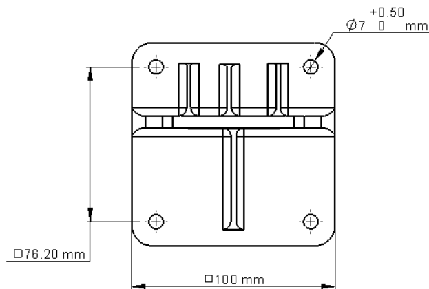
Figure 13: Tilt Mount Base - Front View
