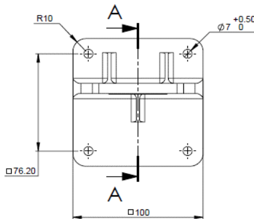
Figure 13: Tilt Mount Base - Plate View
