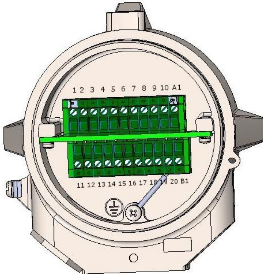
FIGURE 16 – TERMINAL VIEW
