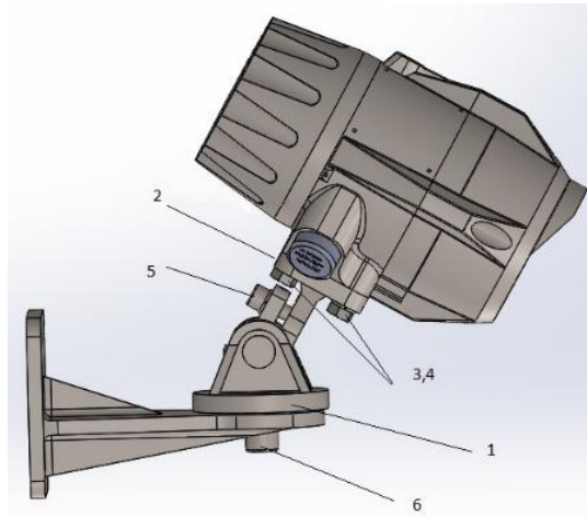
FIGURE 15 - DETECTOR ON TILT MOUNT – SIDE VIEW
