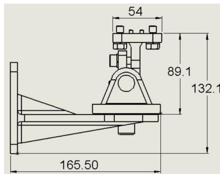
Figure 14: Tilt mount base – Side View
