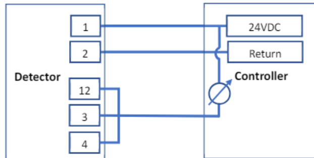
FIGURE 20 – SINK 3-WIRE SCHEME
