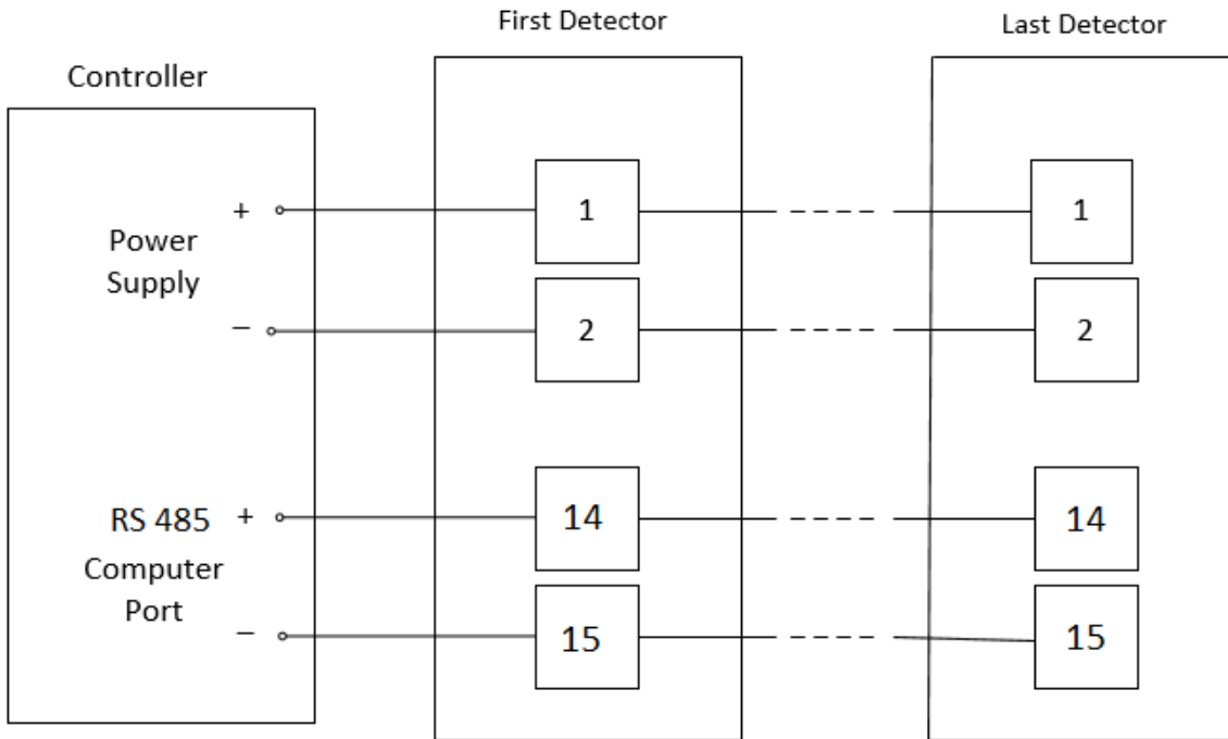
Figure 22 - RS-485 Networking
