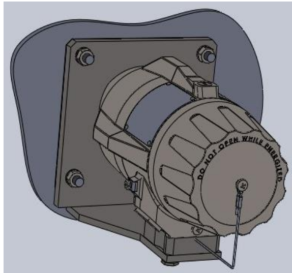
FIGURE 10 - DUCT MOUNT DMW-S02
