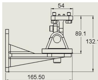
Figure 14 - Tilt mount base – Side View
