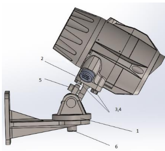
FIGURE 15 - DETECTOR ON TILT MOUNT – SIDE VIEW
