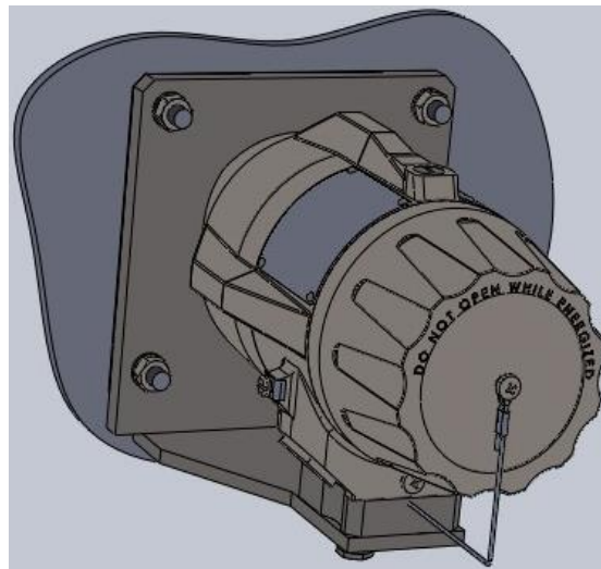
FIGURE 10 - DUCT MOUNT DMW-S02
