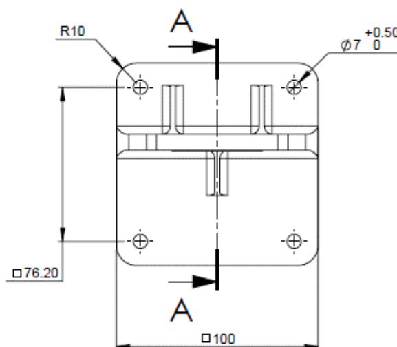
Figure 13 - Tilt Mount Base - Plate View
